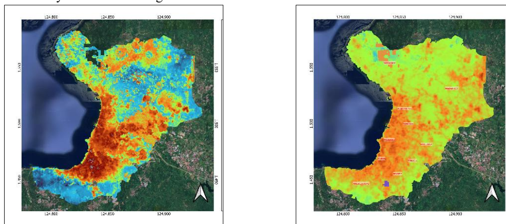
Figure 4 Land Surface Temperature
