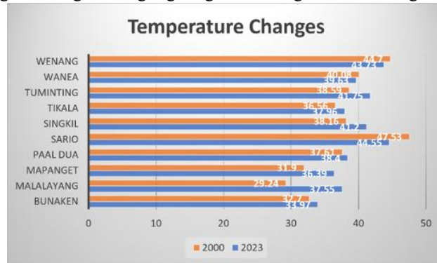
Figure 5 Bar Chart of Temperature Variations Among Subdistricts in Manado City
