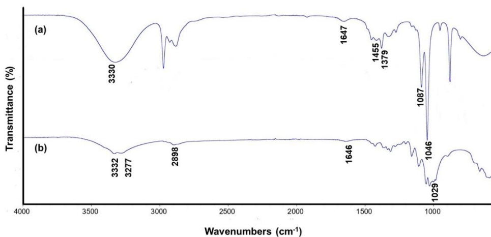
Figure 3. The IR spectra of dithizone (a) and filter paper immobilized by dithizone
