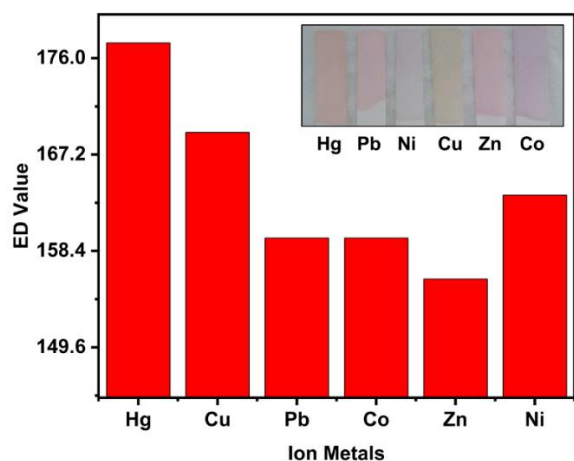
Figure 6. Response of the sensor with other metals in ED value
