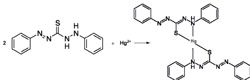
Figure 5. Complex reaction of \text{Hg}^{2+} and dithizone
