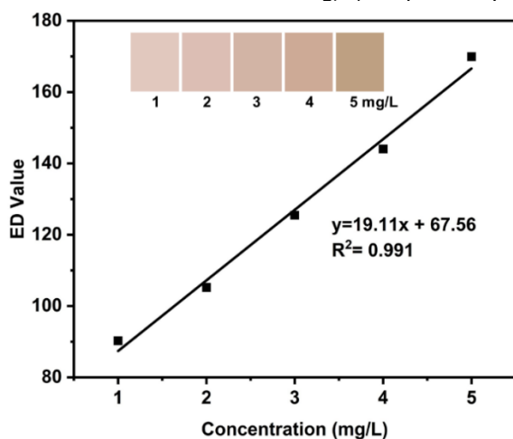
Figure 4. Calibration curve of the paper-based sensor
