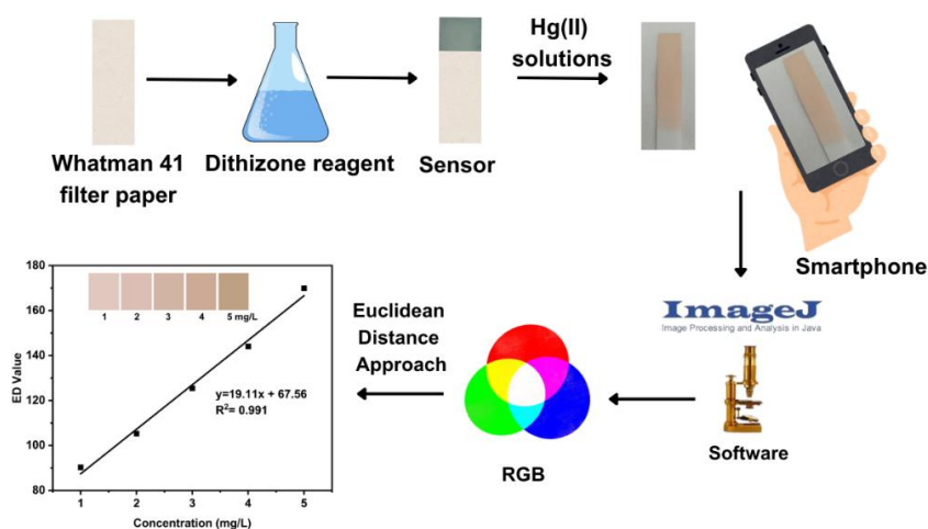
Figure 1. Schematic illustration of paper-based sensor.
