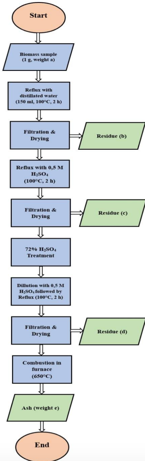
Figure 2. Flow diagram of lignocellulosic composition analysis using the Chesson method.
