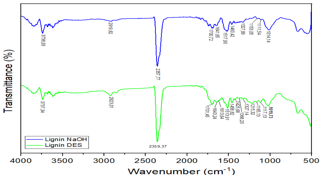
Figure 6. FTIR spectra of lignin NaOH and DES
