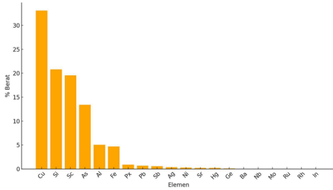
Gambar 3. Hasil analisis XRF sampel
