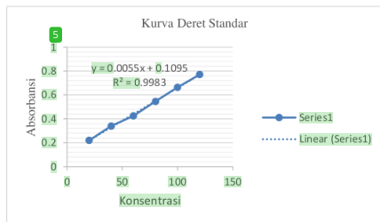
Figure 4.1. Kurva Deret Standar Asam Galat
