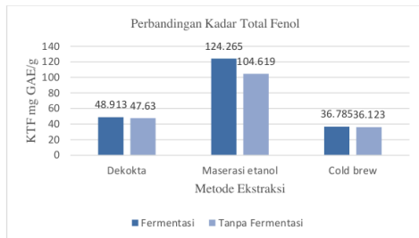
Figure 4.2 . Grafik Perbandingan Kadar Total Fenol
